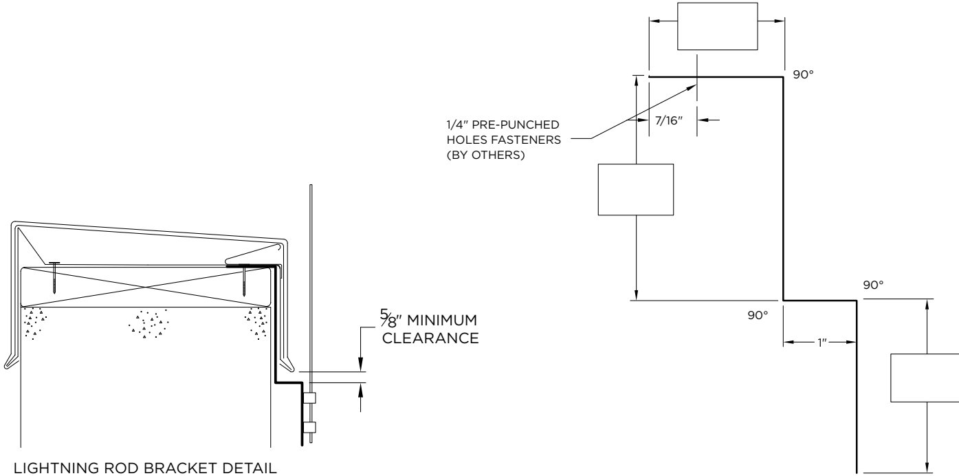
LIGHTNING ROD BRACKET DETAIL
