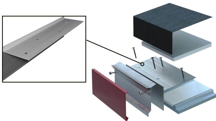
Eliminailer-T shown on flute-filled application featuring Anchor-Tite Drip Edge.
